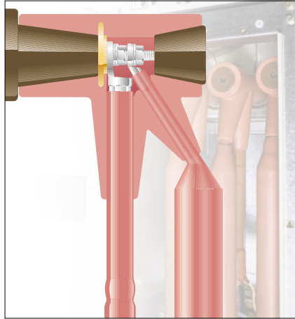
T-adapter for perpendicular connection of termination and surge arrester to SF 6 -insulated switchgear
