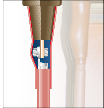
Straight adapter for vertical connection of the termination to SF 6 -insulated switchgear
