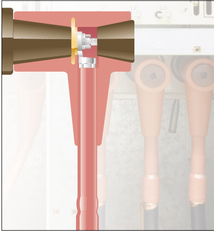
T-adapter for perpendicular connection of the termination to SF 6 -insulated switchgear
