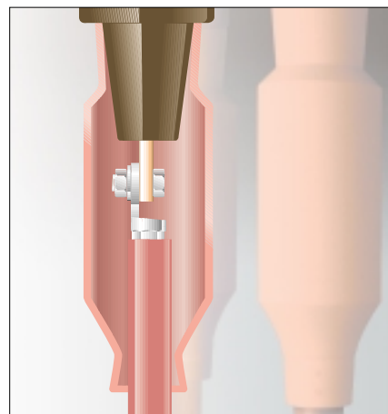
RCAB inline application up to 24 kV
