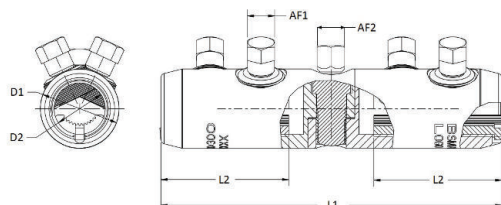
Split Connector
