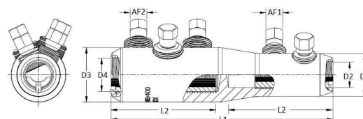
Reduction Connector
