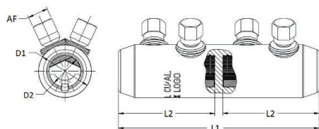
Mechanical Connector
